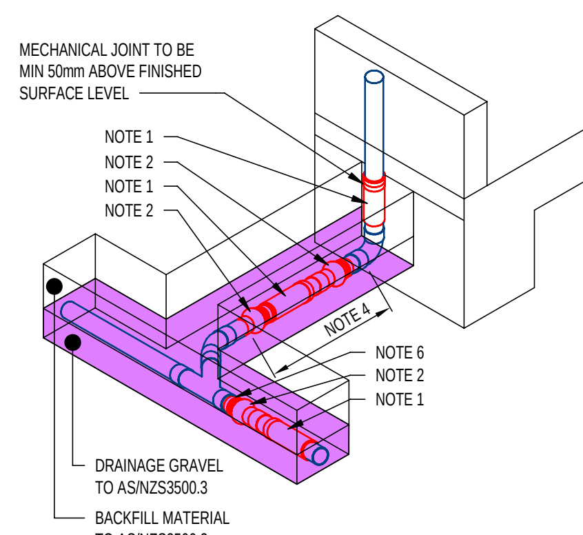
2 STORMWATER DOWNPIPES
