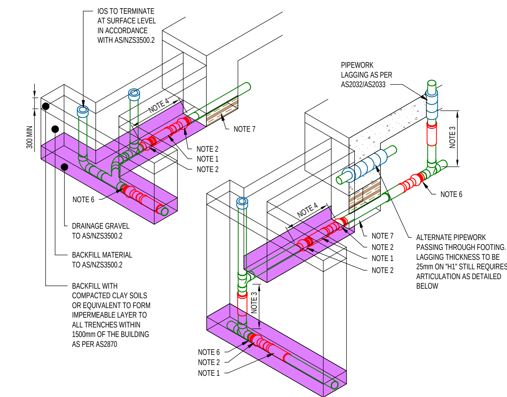
1 IN GROUND DRAINAGE (STORMWATER & SANITARY) NTS
